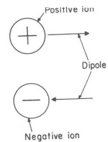
Fig. 2.32. The minimum interaction-energy orientation of a dipole to an ion.
