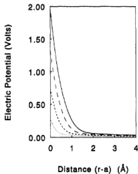
Figure 2. Effect of fractional surface charge density on computed electric potential profiles for K^+ in water at 298 K: (···) 40% (of final surface charge); (---) 60%; (--) 80%; (—) 100%.
