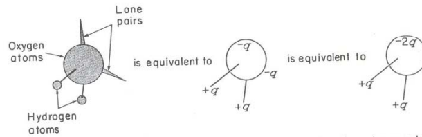
Fig. 2.45. The electrical equivalence between a water molecule and a quadrupole.
