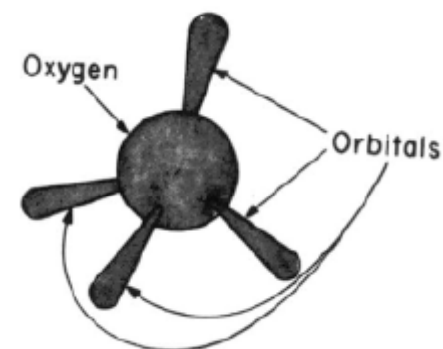
Fig. 2.6. The hybrid orbitals of an oxygen atom.
