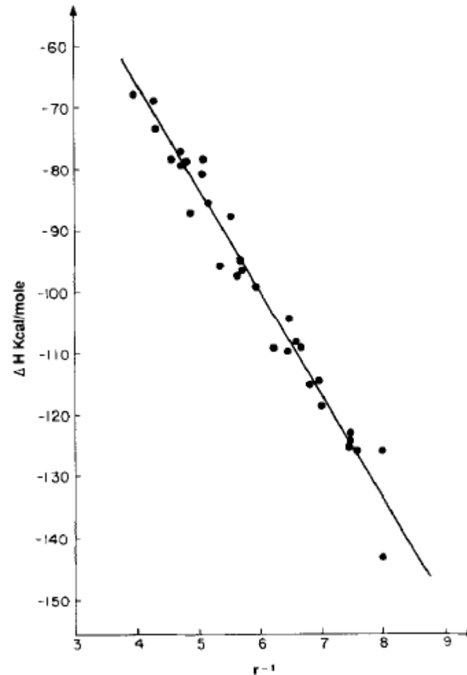
FIGURE 1. Comparison of experimental (dots) and predicted (solid line) enthalpies of ion hydration. The enthalpies are given per unit charge. The experimental values are given for the following ions: \text{Li}^+ , \text{Na}^+ , \text{K}^+ , \text{Rb}^+ , \text{Cs}^+ , \text{F}^- , \text{Cl}^- , \text{Br}^- , \text{I}^- , \text{Cu}^+ , \text{Ag}^+ , \text{Cu}^{+2} , \text{Mg}^{+2} , \text{Ca}^{+2} , \text{Sr}^{+2} , \text{Ba}^{+2} , \text{Zn}^{+2} , \text{Cd}^{+2} , \text{Hg}^{+2} , \text{Al}^{+3} , \text{Sc}^{+3} , \text{Y}^{+3} , \text{La}^{+3} , \text{Ce}^{+3} , \text{Ce}^{+4} , \text{Ga}^{+3} , \text{In}^{+3} , \text{NH}_4^+ , \text{OH}^- , \text{S}^{-2} , \text{SH}^- .
