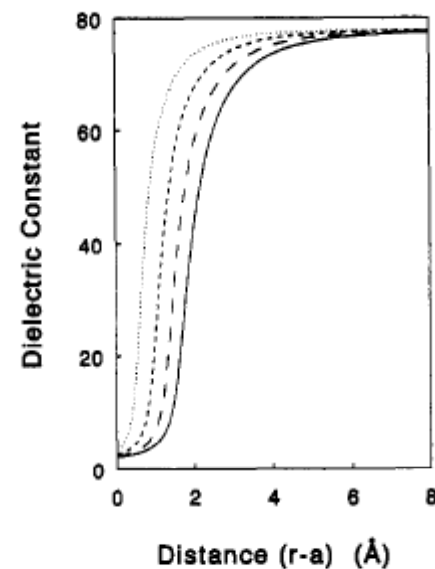
Figure 3. Effect of fractional surface charge density on the computed solvent dielectric profiles for K^+ in water at 298 K: (···) 40% (of final surface charge); (---) 60%; (--) 80%; (—) 100%.
