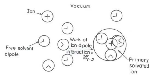
Fig. 2.33. Formation of a primary solvated ion.
