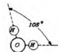
Fig. 2.5. A water molecule is nonlinear.
