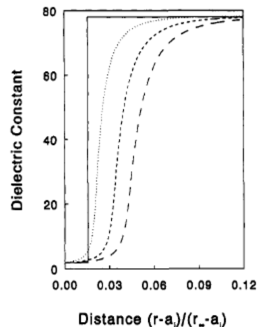
Figure 6. Radial variation in the predicted solvent dielectric profile for uni- and multivalent cations in water at 298 K: (···) \text{Na}^+ ; (---) \text{Ca}^{2+} ; (-·-) \text{Y}^{3+} ; (—) one-layer profile of Abraham and Lizzi. 8
