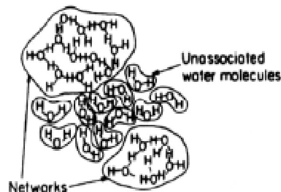
Fig. 2.10. Schematic diagram to show that in liquid water there are networks of associated water molecules and also a certain fraction of free, unassociated water molecules.
