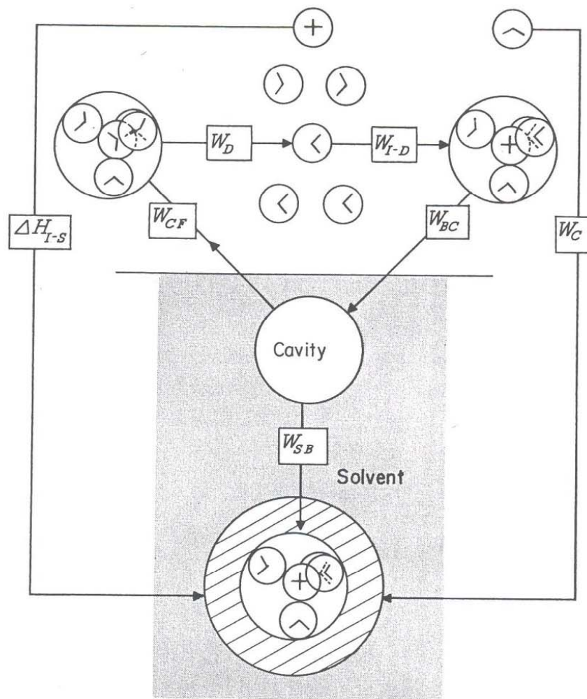
Fig. 2.38. How the total heat \Delta H_{I-S} of ion-solvent interactions has been separated in a thought experiment into the various steps of cavity formation W_{CF} , cluster dissociation W_D , formation of primary solvated ion W_{I-D} , Born charging W_{BC} , structure breaking W_{SB} , and condensation, W_C .
