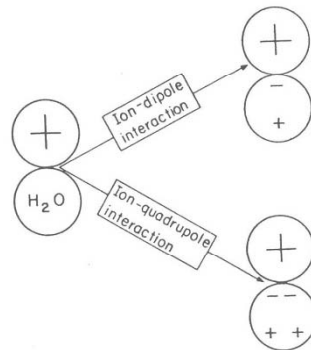
Fig. 2.46. Improvement in the calculation of the ion-water molecule interactions by altering the model of the water molecule from a dipole to a quadrupole.
