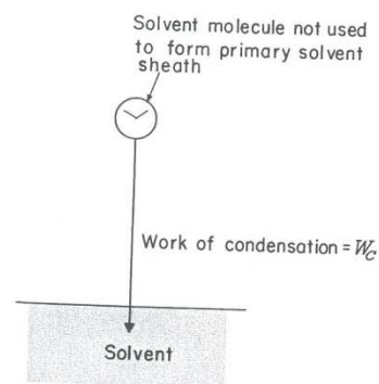
Fig. 2.37. The condensation of a water molecule left behind in vacuum because it was not used to form the primary solvent sheath.
