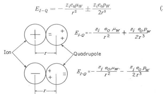
Fig. 2.47. The symmetrical orientation of a quadrupole to an ion.
