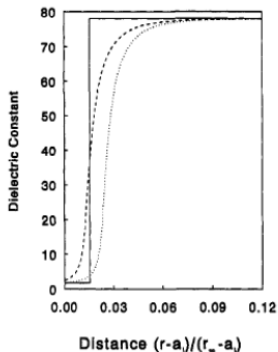
Figure 5. Radial variation in the predicted solvent dielectric profile for univalent cations in water at 298 K: (···) \text{Li}^+ ; (---) \text{Cs}^+ ; (—) one-layer profile of Abraham and Lizzi. 8
