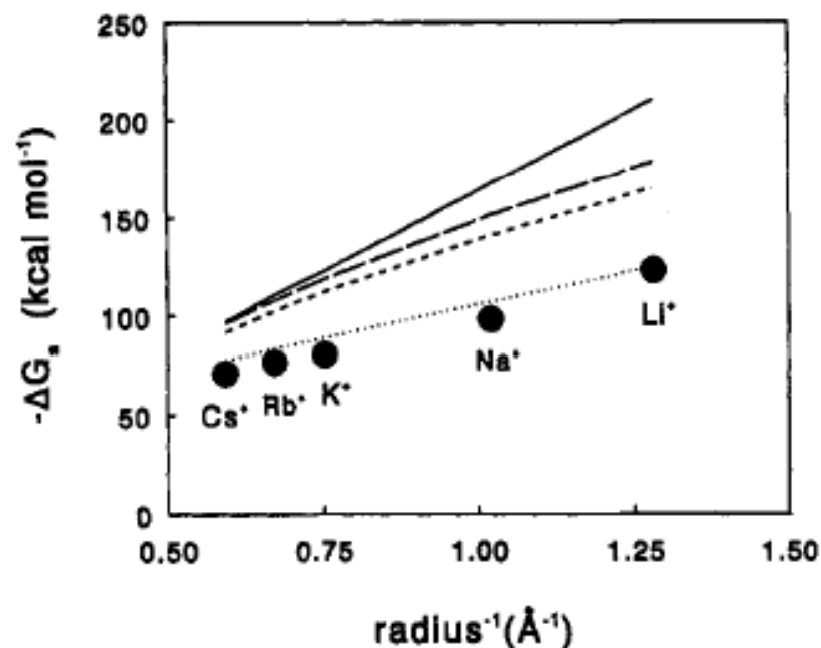
Figure 4. Comparison of hydration free energies for alkali metal ions at 298 K: (●) experimental data (from ref 22); (···) present theory; (---) theory of Markin and Volkov; 13 (---) theory of Laidler and Pegis; 14 (—) Born theory. 1
