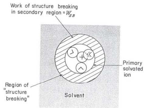
Fig. 2.36. The introduction of a primary solvated ion into the cavity causes disturbance to the structure of the solvent in the immediate vicinity of the solvated ion.
