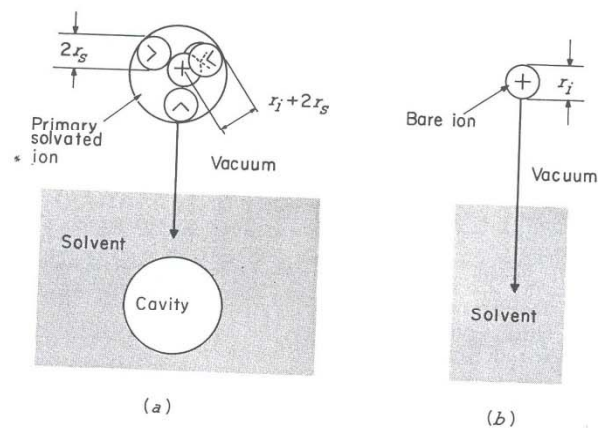
Fig. 2.35. The difference between the Born charging process in (a) the ion-dipole model of solvation in which a primary solvated ion of radius r_i + 2r_s is transferred into the solvent (Section 2.3.3) and in (b) the nonstructural model of Born (cf. Section 2.2.5) in which a bare ion of radius r_i is involved.
